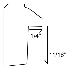
WM281 11/16" x 1-1/8"
