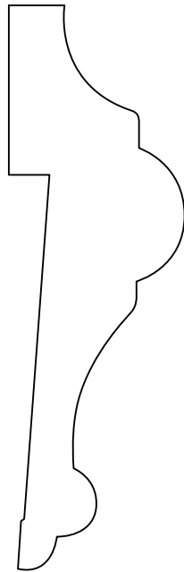
RAB297 1-1/16" x 3-1/4" (Rabbeted Chair Rail)
