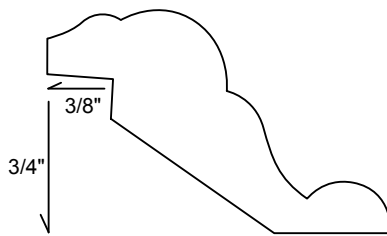
ES11 1-1/8" x 1-3/4" (Rabbeted Panel)
