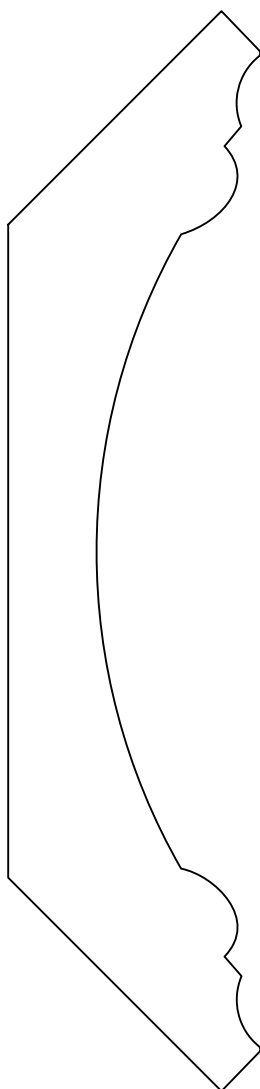
DCR558PP 1-5/16" x 5-5/8"
